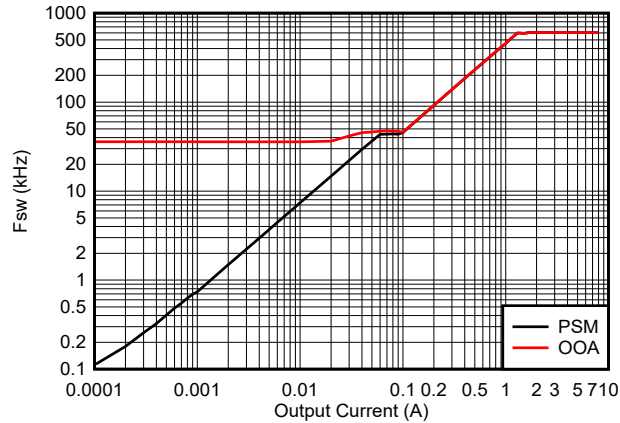
Figure 6-7. TPS51383 Fsw vs Iout
