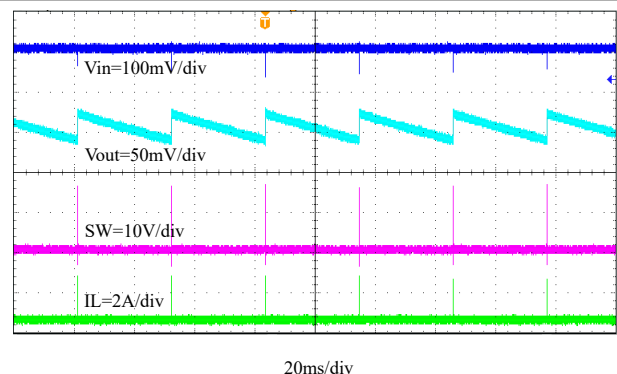
Figure 8-7. PSM Mode Output Voltage Ripple, Iout = 0 A
