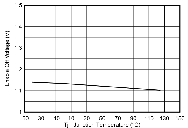
Figure 6-12. Enable Off Voltage vs Temperature
