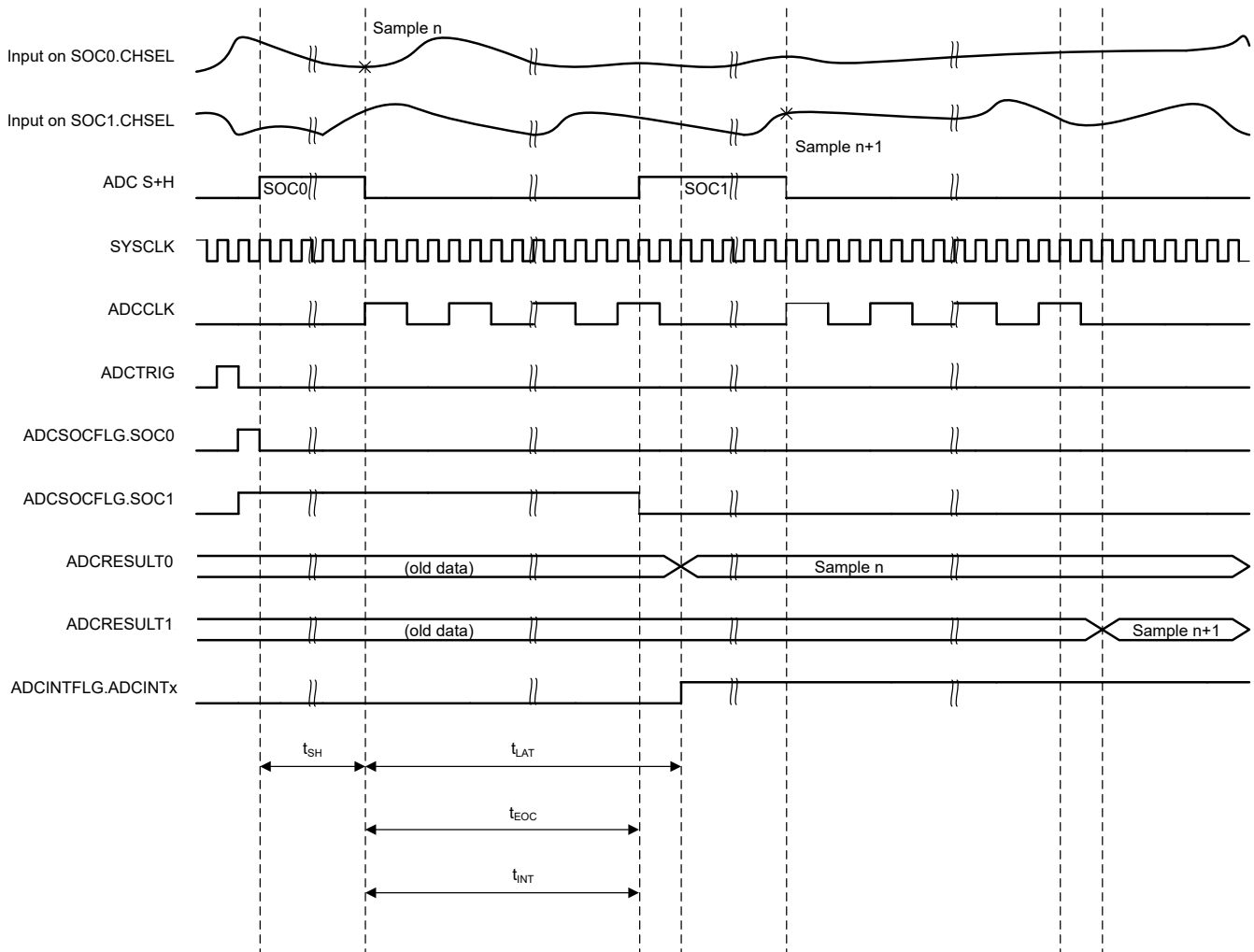
Figure 6-40. ADC Timings
