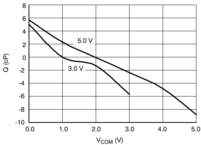
Figure 6. Charge Injection
