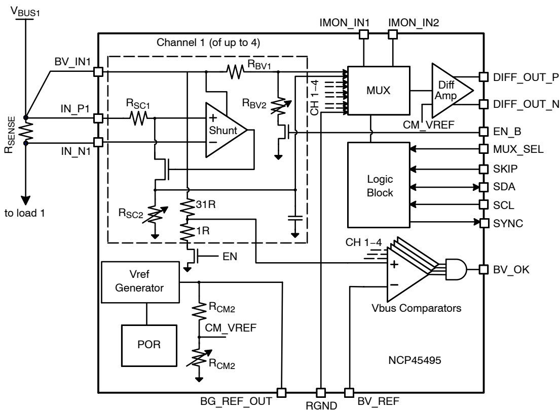
Figure 1. Block Diagram
