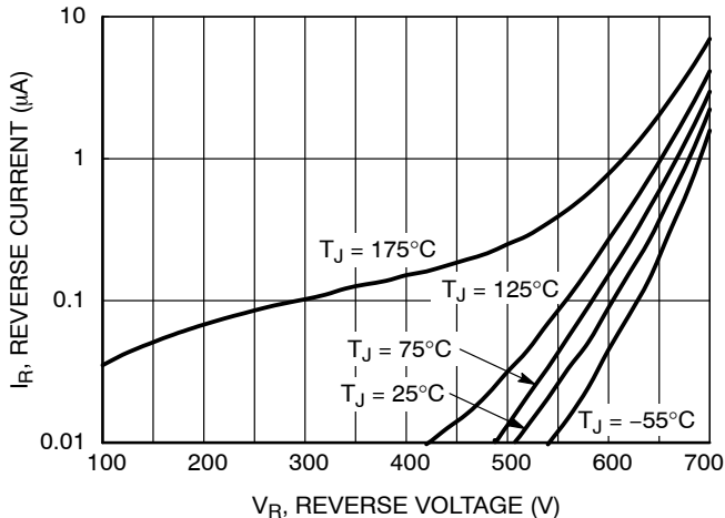
Figure 22. Typical Reverse Current vs. Reverse Voltage
