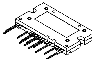
APMCD-A16 12 LEAD CASE MODGG
