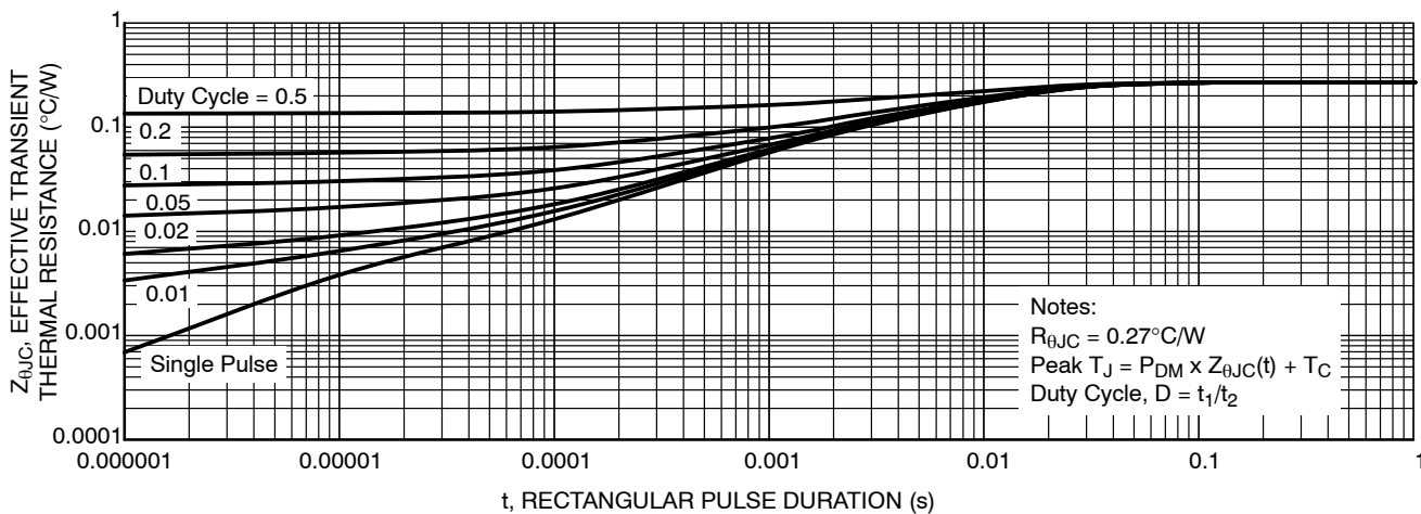
Figure 24. Transient Thermal Impedance
